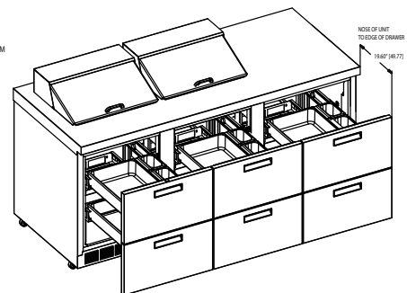
D4472N-12 ISO VIEW
