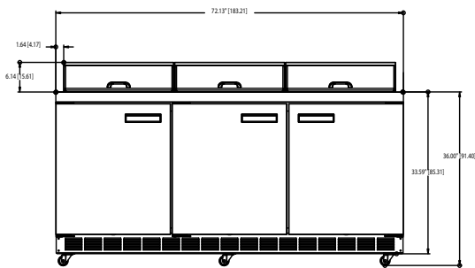
4472N-18 ELEVATION VIEW
