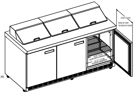
4472N-18 ISO VIEW
