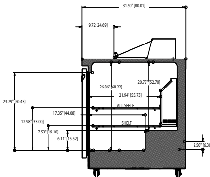
4472N-18 RIGHT SIDE VIEW
