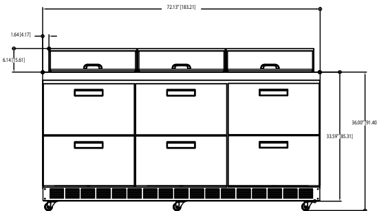
D4472N-18 ELEVATION VIEW
