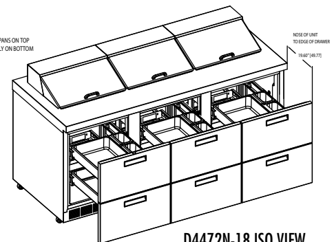
D4472N-18 ISO VIEW
