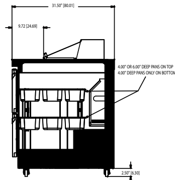
D4472N-12 RIGHT SIDE VIEW
