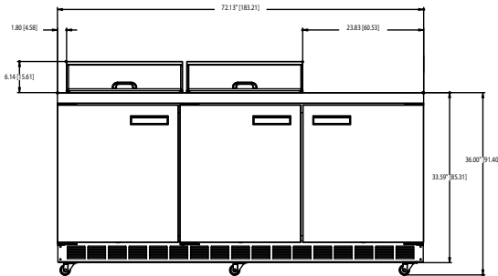
4472N-12 ELEVATION VIEW
