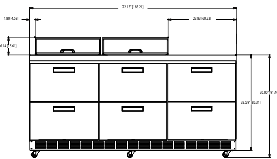
D4472N-12 ELEVATION VIEW
